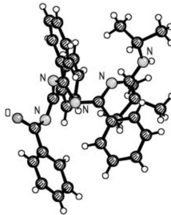
Figure 8. Molecular structure of 14 in the solid state. Bond parameters are not given because of low crystal quality.
