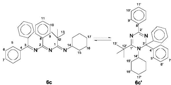
Scheme 14. Numbering of 6c/6c' for NMR assignment.
