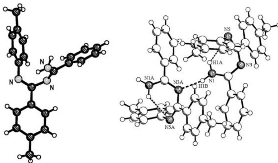
Figure 1. Molecular structure of 1b in the solid state (left: single molecule; right: two molecules with hydrogen bonding shown). Selected structural parameters: bond lengths [Å]: N1–C2 1.288(2), C2–N3 1.411(2), N3–C4 1.294(2), C4–N5 1.350(2); bond angles [°]: N1–C2–C3 124.32(13), C2–N3–C4 118.26(11), N3–C4–N5 125.30(13); torsional angles [°]: N1–C2–N3–C4–N5 72.04, C2–N3–C4–N5 6.99.
