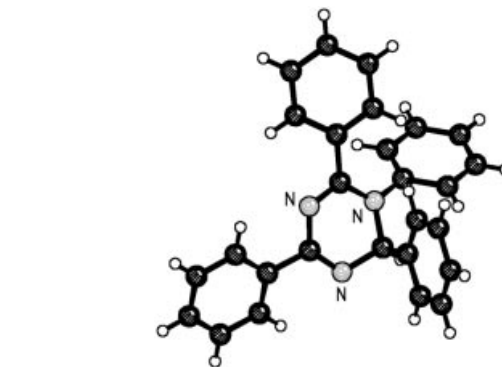
Figure 3. Molecular structure of 3a in the solid state. Selected structural parameters: bond lengths [Å]: N1–C2 1.463(1), C2–N3 1.480(1), N3–C4 1.363(1), C4–N5 1.306(1); bond angles [°]: N1–C2–C3 110.63(8), C2–N3–C4 115.58(8), N3–C4–N5 121.79(9), C4–N5–C6 115.42(8), N5–C6–N1 126.65(9); torsional angles [°]: N1–C2–N3–C4 42.75, C2–N3–C4–N5 –19.83, N3–C4–N5–C6 –11.42, C4–N5–C6–N1 20.36, N5–C6–N1–C2 4.97.
