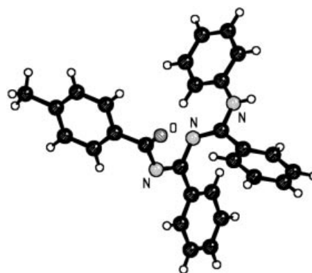
Figure 5. Molecular structure of 8a in the solid state. Selected structural parameters: bond lengths [Å]: O1–C2 1.221(4), C2–N3 1.391(4), N3–C4 1.294(4), C4–N5 1.388(4), N5–C6 1.291(4), C6–N7 1.363(4); bond angles [°]: O1–C2–C3 121.6(3), C2–N3–C4 121.1(3), N3–C4–N5 121.2(3), C4–N5–C6 123.4(3), N5–C6–N7 121.3(3); torsional angles [°]: O1–C2–N3–C4 –69.21, C2–N3–C4–N5 –13.76, N3–C4–N5–C6 120.56, C4–N5–C6–N7 172.91.
