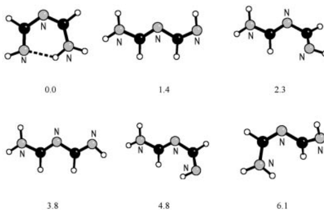
Figure 2. DFT-optimized structures for 1,3,5-triazapenta-1,3-diene isomers with relative energies [kcal/mol], B3LYP/6-31+G(d,p) (incl. ZPE).
