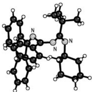
Figure 4. Molecular structure of 6b in the solid state. Selected structural parameters: bond lengths [Å]: N1–C2 1.265(2), C2–N3 1.420(2), N3–C4 1.279(2), C4–N5 1.404(2), N5–C6 1.276(2); bond angles [°]: N1–C2–C3 125.3(2), C2–N3–C4 119.1(1), N3–C4–N5 120.8(1), C4–N5–C6 124.0(1); torsional angles [°]: N1–C2–N3–C4 –100.4, C2–N3–C4–N5 –0.2, N3–C4–N5–C6 104.6.
