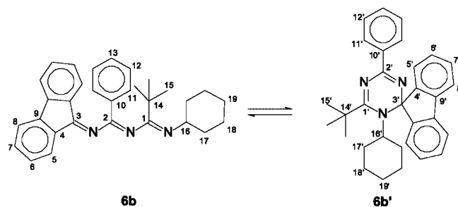
Scheme 13. Numbering of 6b/6b' for NMR assignment.
